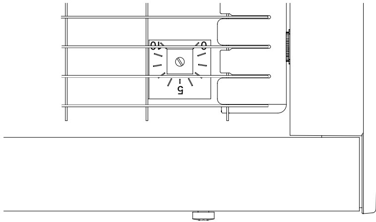
Fig. 2: Stepless airflow control. Internal potentiometer (accessible through the outlet grille).
